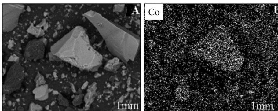
Fig. 2. SEM image (a) and EDS mapping of Co (b) for \text{SiO}_2/\text{C}/\text{CoPc} .
