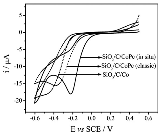
Fig. 4. Cyclic voltammograms obtained for: \text{SiO}_2/\text{C}/\text{CoPc} -in situ electrode (solid line), \text{SiO}_2/\text{C}/\text{CoPc} -classically electrode (dotted line) and \text{SiO}_2/\text{C}/\text{Co} electrode (dashed line), all in the presence of 8.2 \text{ mg L}^{-1} \text{ O}_2 . Experimental conditions: T = 298 \text{ K} , \nu = 10 \text{ mV s}^{-1} ; 1 \text{ mol L}^{-1} \text{ KCl} , \text{pH} = 7 .
