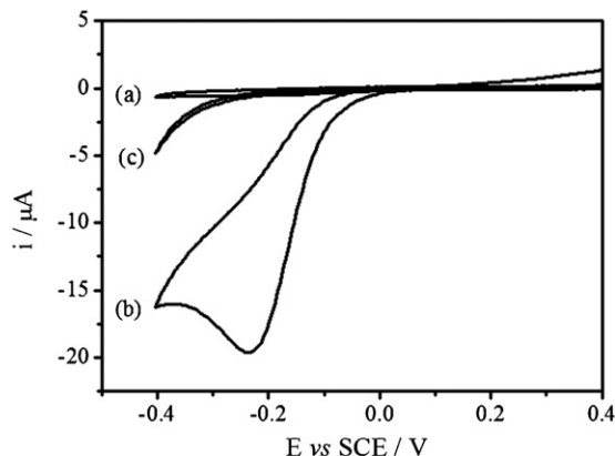
Fig. 3. Cyclic voltammograms for: \text{SiO}_2/\text{C}/\text{CoPc} electrode in the absence (a) and presence of \text{O}_2 (b) and voltammogram of \text{SiO}_2/\text{C} bare electrode in the presence of \text{O}_2 (c) in the concentration of 9.1 \text{ mg L}^{-1} \text{ O}_2 . Experimental conditions: T = 298 \text{ K} , scan rate \nu = 10 \text{ mV s}^{-1} ; 1 \text{ mol L}^{-1} \text{ KCl} ; \text{pH} = 7 .
