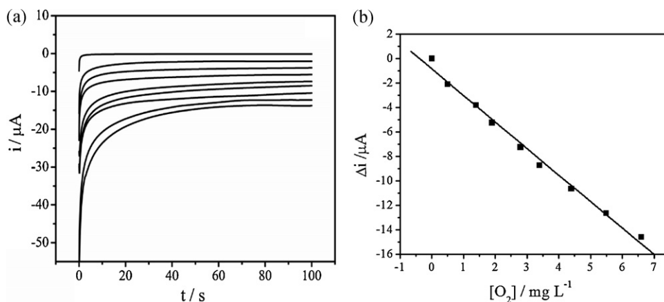
Fig. 8. (a) Amperometry response of the SiO 2 /C/CoPc electrode in different oxygen concentrations (mg L -1 ): from top to bottom: 0.0, 0.5, 1.4, 1.9, 2.8, 3.4, 4.4, 5.5, 6.6. (b) Plot of cathodic current ( \Delta i_{cp} ) versus [O 2 ] (measured at 50 s). Experimental conditions: T = 298 K, E_{appl} = -0.23 V; 1 mol L -1 KCl; pH 7.
