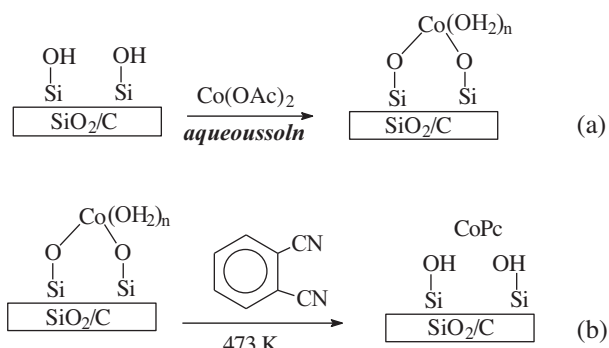
Scheme 1. In situ generation of cobalt phthalocyanine (CoPc) inside the pores of \text{SiO}_2/\text{C} : Si–OH Brønsted acid sites in the pores of the matrix: (a) adsorption of Co(II) on the surface through Si–O–Co bond formation and (b) generation of CoPc inside the pore.
