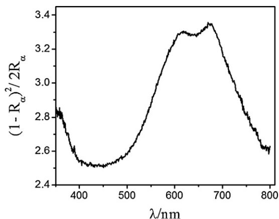
Fig. 1. UV-vis diffuse reflectance spectra of \text{SiO}_2/\text{C}/\text{CoPc} , expressed in Kubelka–Munk units.
