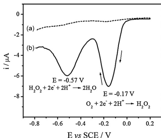
Fig. 6. Differential pulse voltammetry measurement of \text{SiO}_2/\text{C}/\text{CoPc} electrode in the absence (a) and presence (b) of 9.0 \text{ mg L}^{-1} \text{ O}_2 . Experimental conditions: T = 298 \text{ K} ; 1 \text{ mol L}^{-1} \text{ KCl} ; \text{pH} = 7 ; \nu = 10 \text{ mV s}^{-1} .
