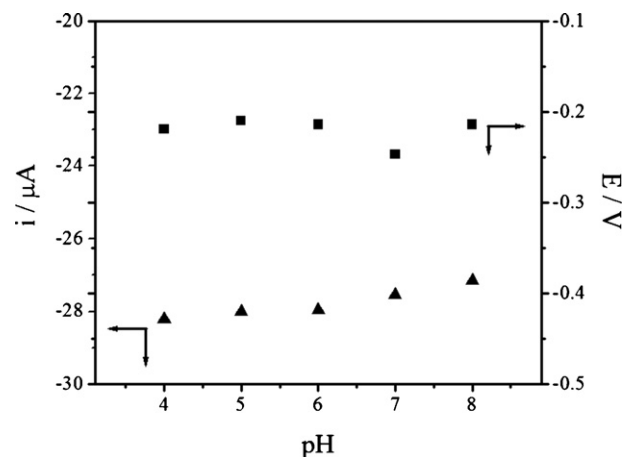
Fig. 7. Values of cathodic peak current and reduction peak potential at a function of the solution pH obtained for the \text{SiO}_2/\text{C}/\text{CoPc} electrode. [\text{O}_2] = 9.0 \text{ mg L}^{-1} ; T = 298 \text{ K} , and \nu = 10 \text{ mV s}^{-1} .
